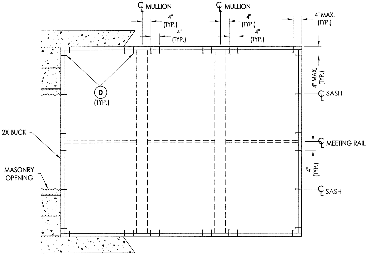
BUCK ANCHORING
